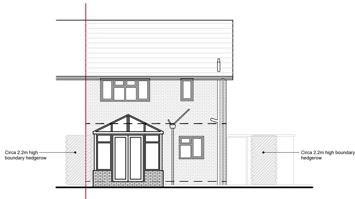
EXISTING NORTHEAST (REAR) ELEVATION 1:100
