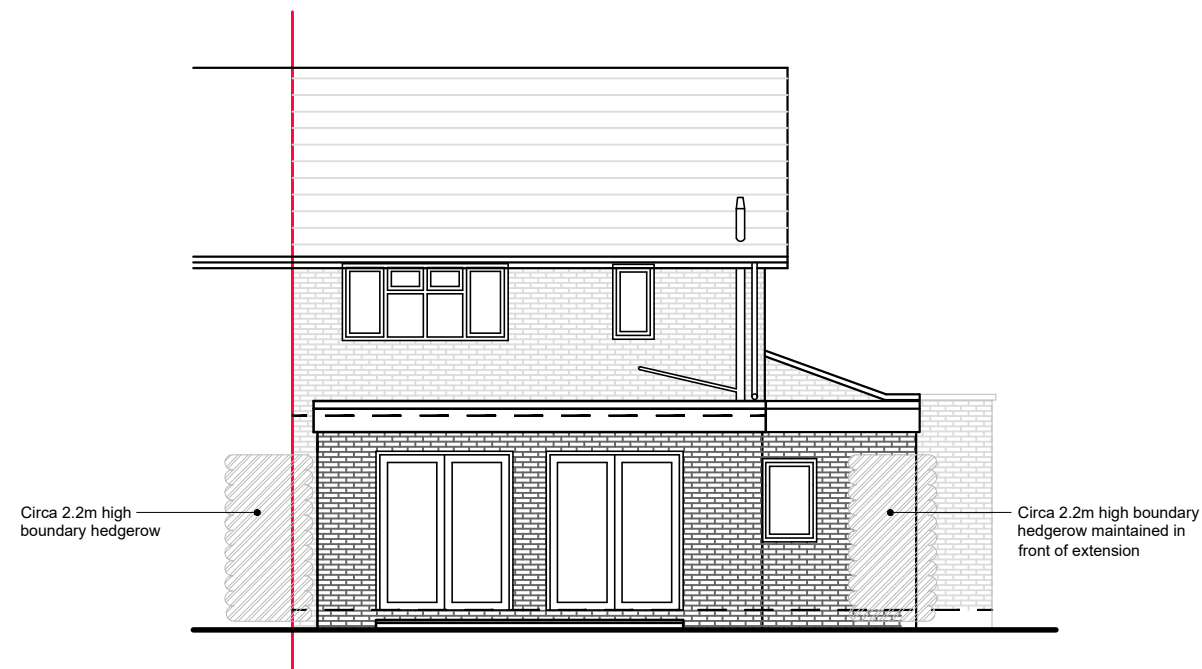
PROPOSED NORTHEAST (REAR) ELEVATION 1:100
