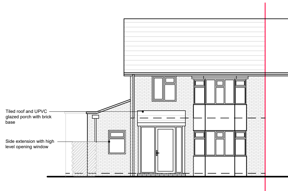
PROPOSED SOUTHWEST (FRONT) ELEVATION 1:100
