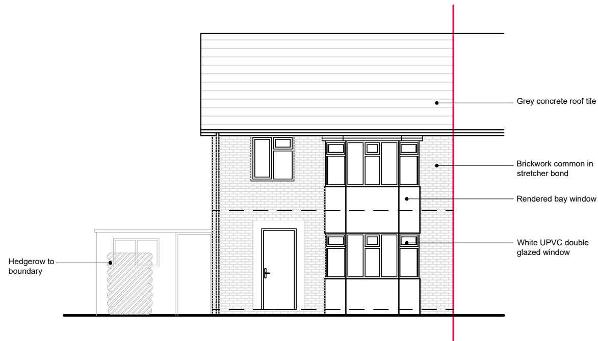
EXISTING SOUTHWEST (FRONT) ELEVATION 1:100
