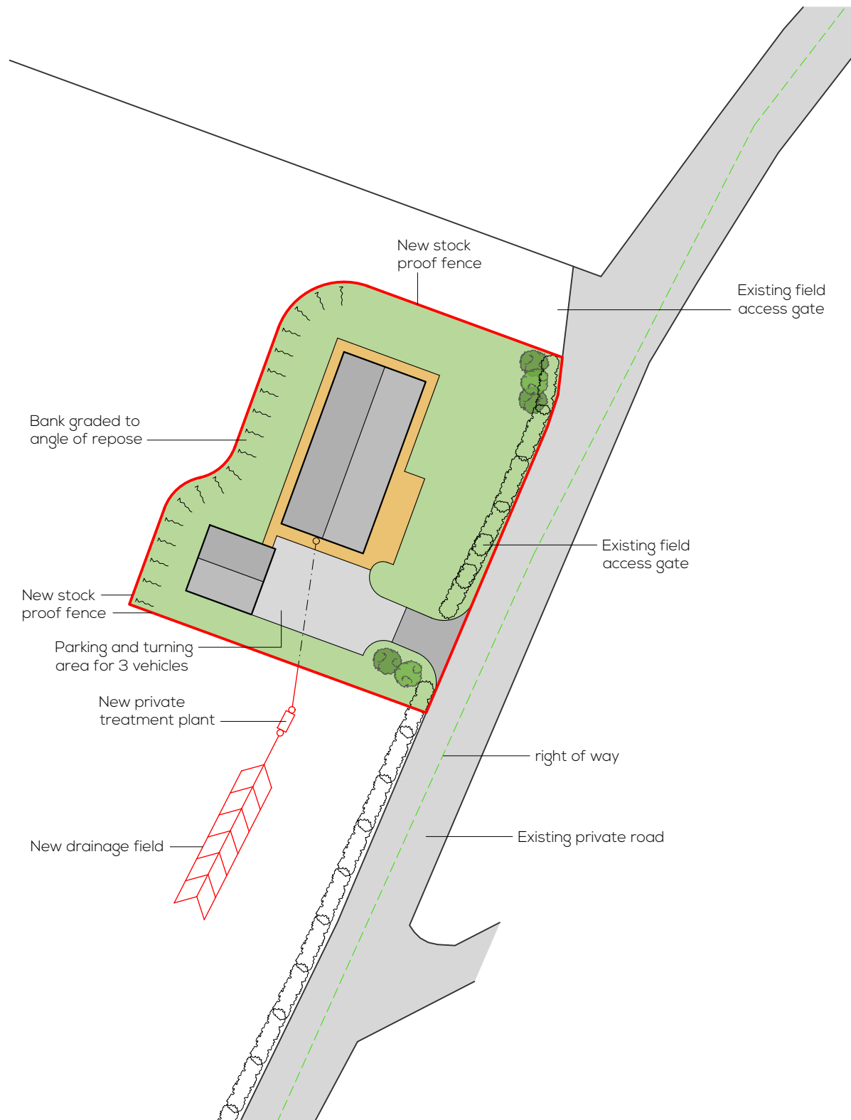
Block Plan - 1:500
