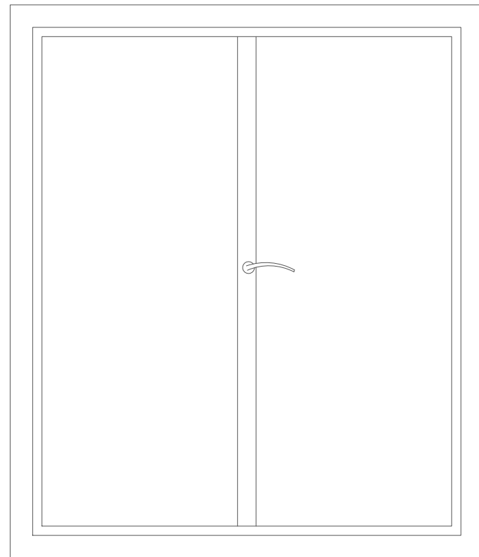
Aluminium inward opening french door
