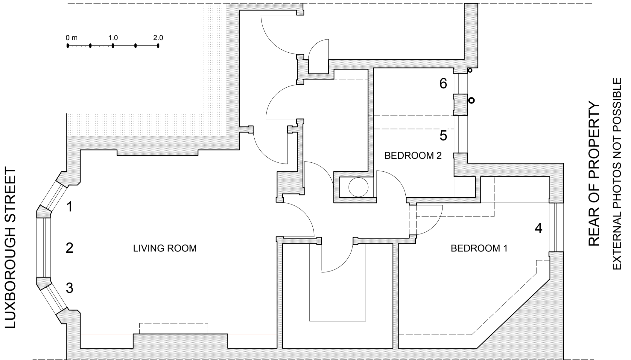
APARTMENT PLAN - SECOND FLOOR - 1:50 SCALE - EXISTING AND PROPOSED
