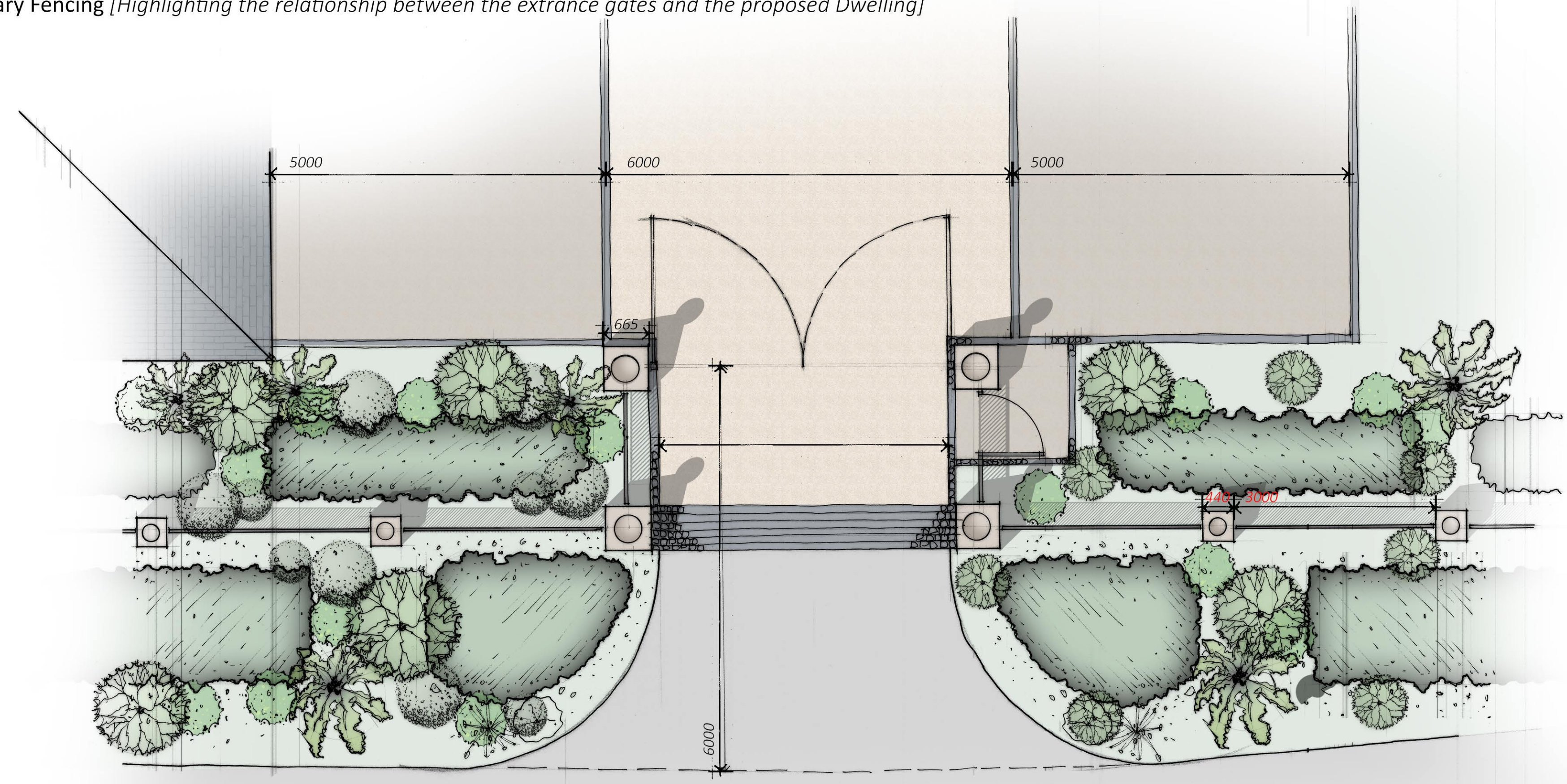
Proposed Entrance Gates Block Plan [Highlighting the relationship between the entrance gates and the proposal] [scale 1:50]
