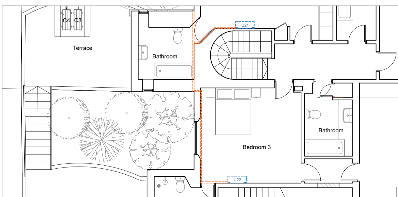
Key plan (Second floor) @ 1:100
