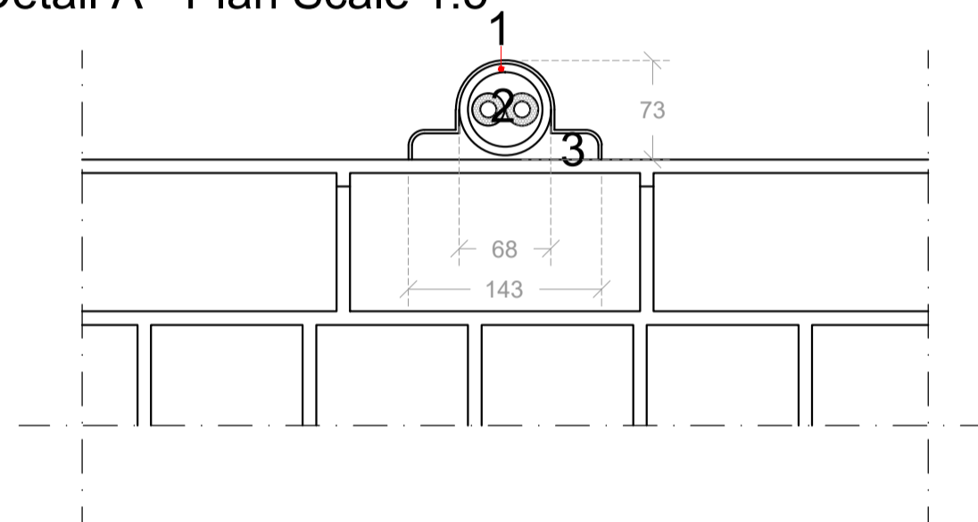
Detail A - Plan Scale 1:5
