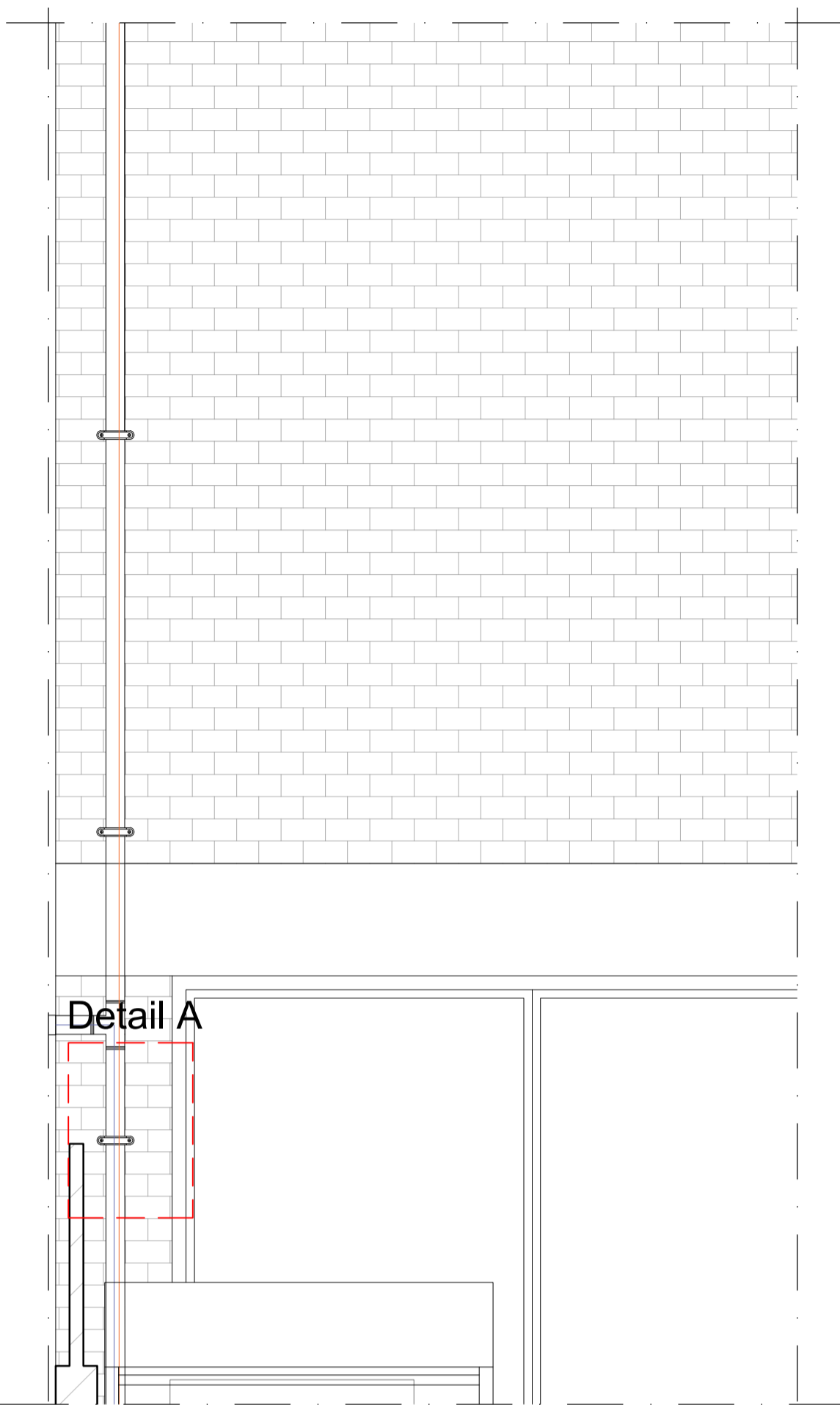
External ducts work enclosure Scale 1:20
