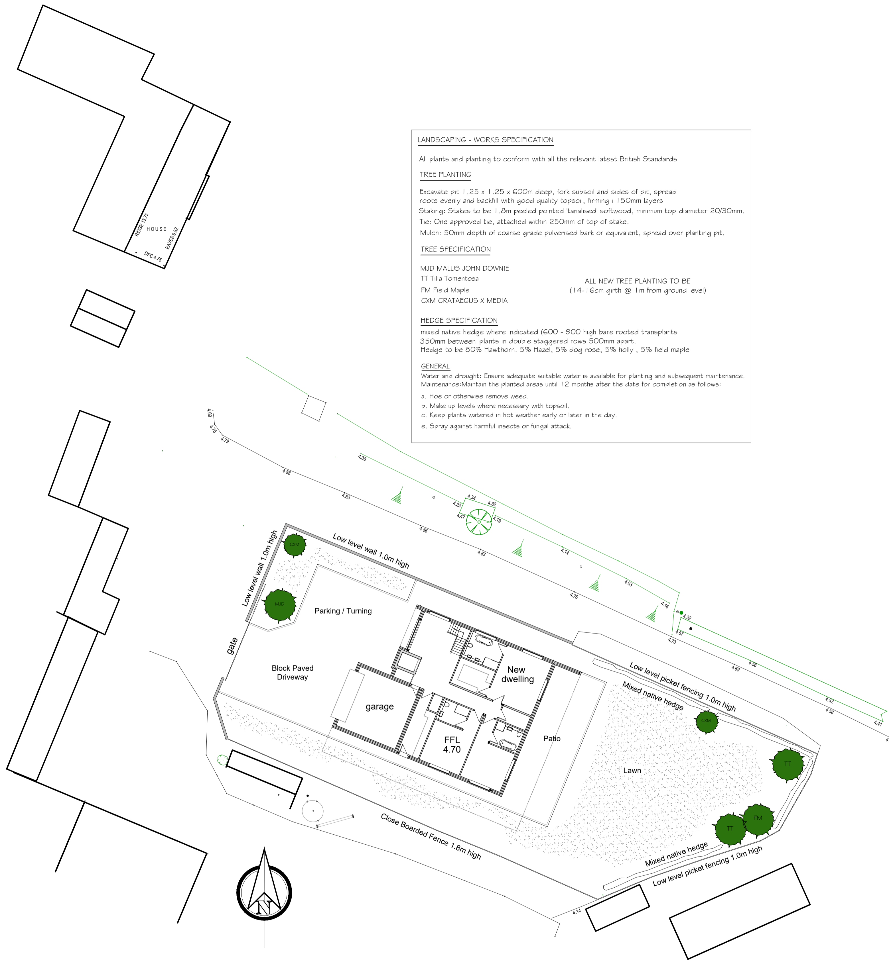
Proposed Site Plan - (scale 1:200)
