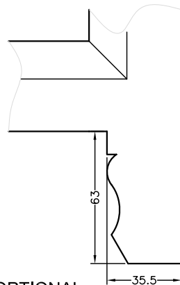
OPTIONAL SASH HORN
