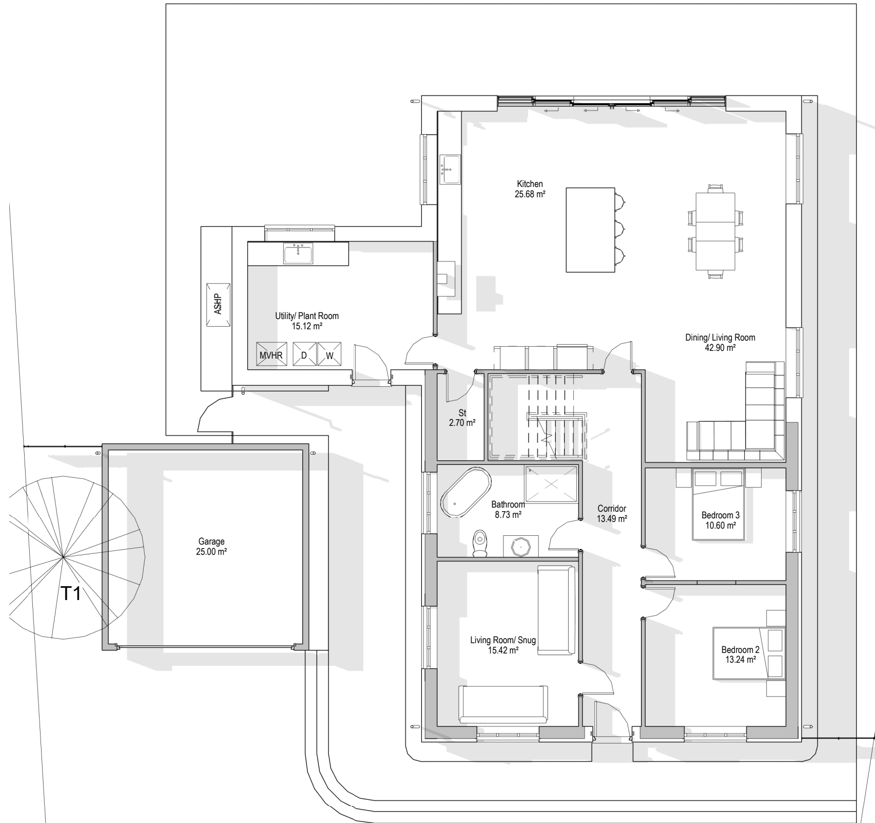
1 Ground Floor - Proposed 1 : 100
