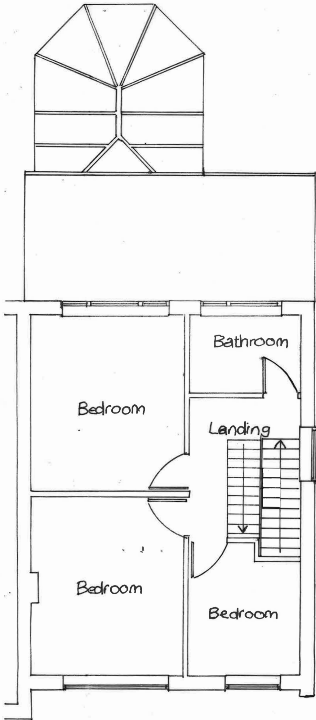
Existing First Floor Plan 1:50
