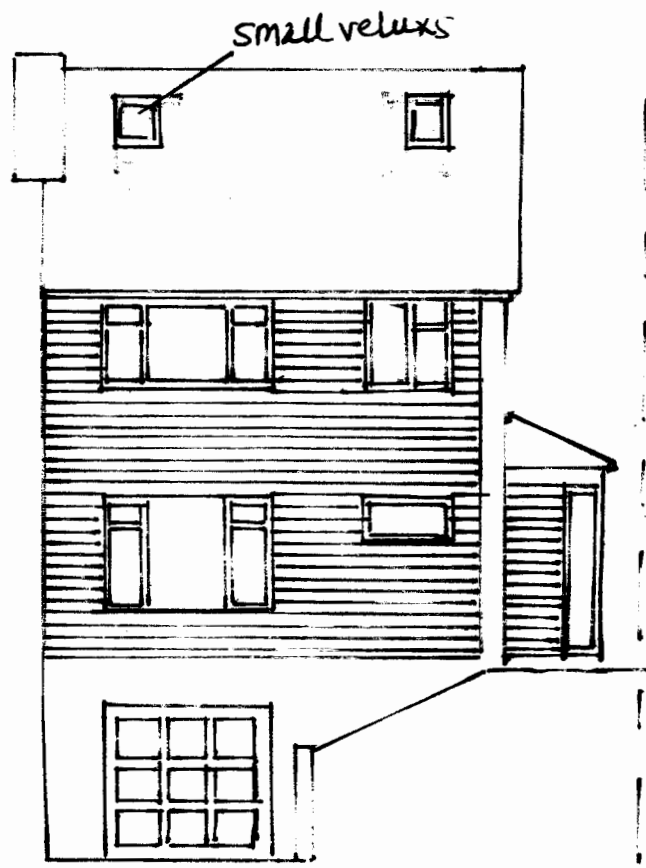
1:100 PROPOSED FRONT ELEVATION
