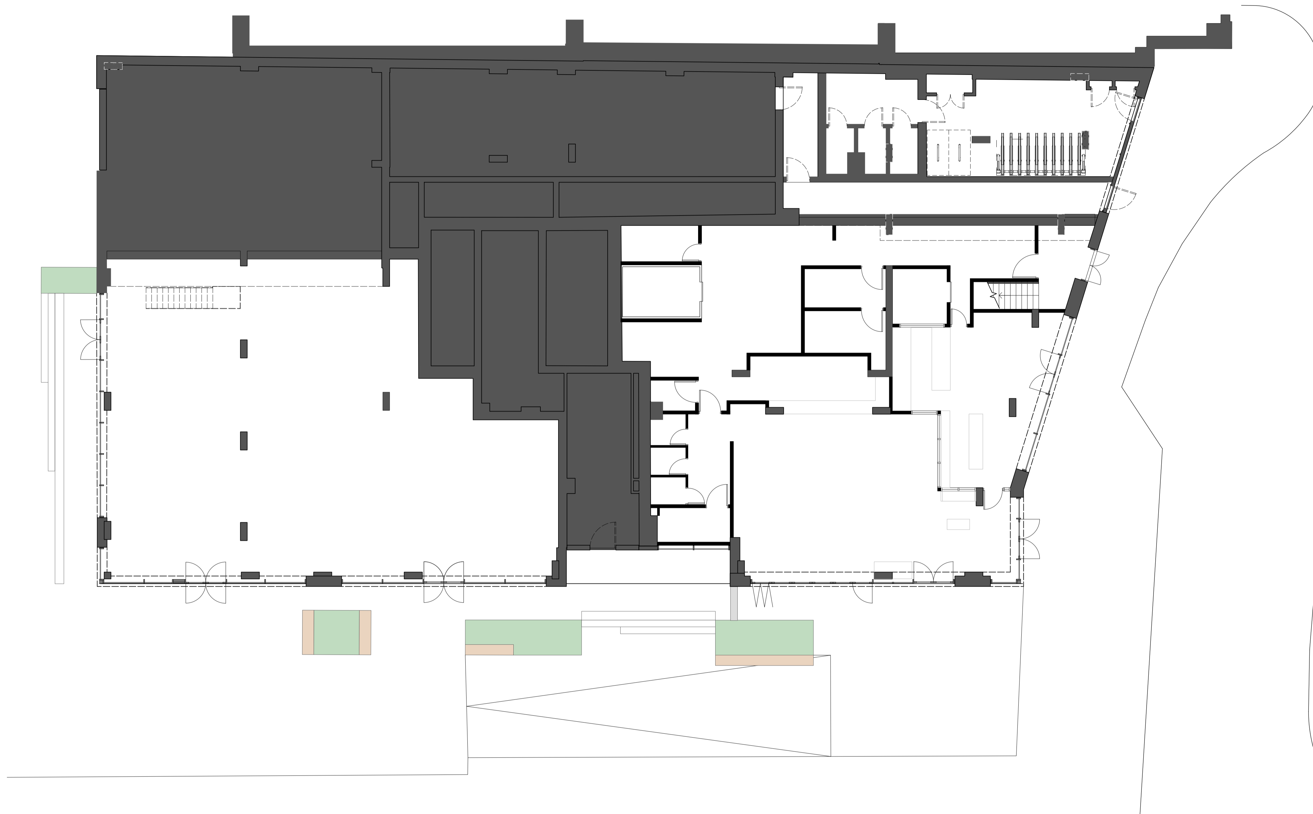
1 Ground Floor Plan Unit 2.3 and 2.4 Scale: 1:100
