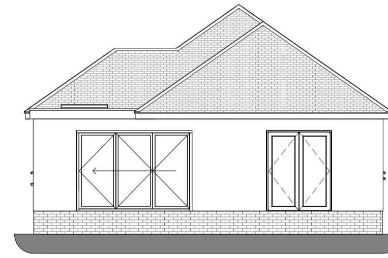
8 Proposed Rear Elevation 1:100
