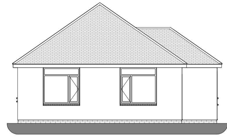
4 Proposed Front Elevation 1:100
