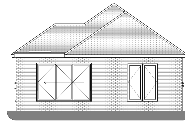
7 Existing Rear Elevation 1:100
