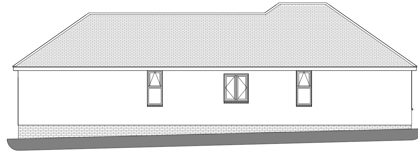
6 Proposed NE Side Elevation 1:100
