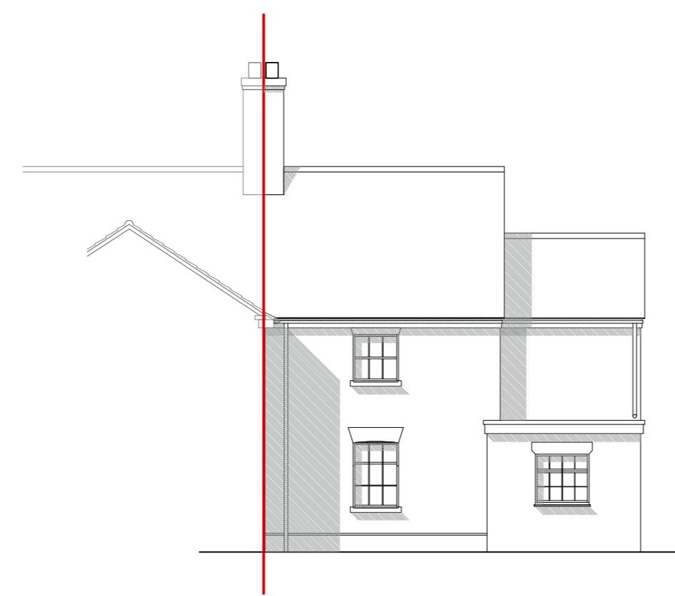
6 EXISTING REAR (NORTH) ELEVATION 1:100
