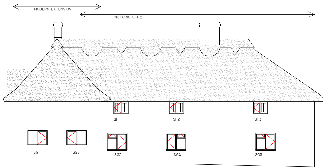
SOUTH ELEVATION EXISTING
