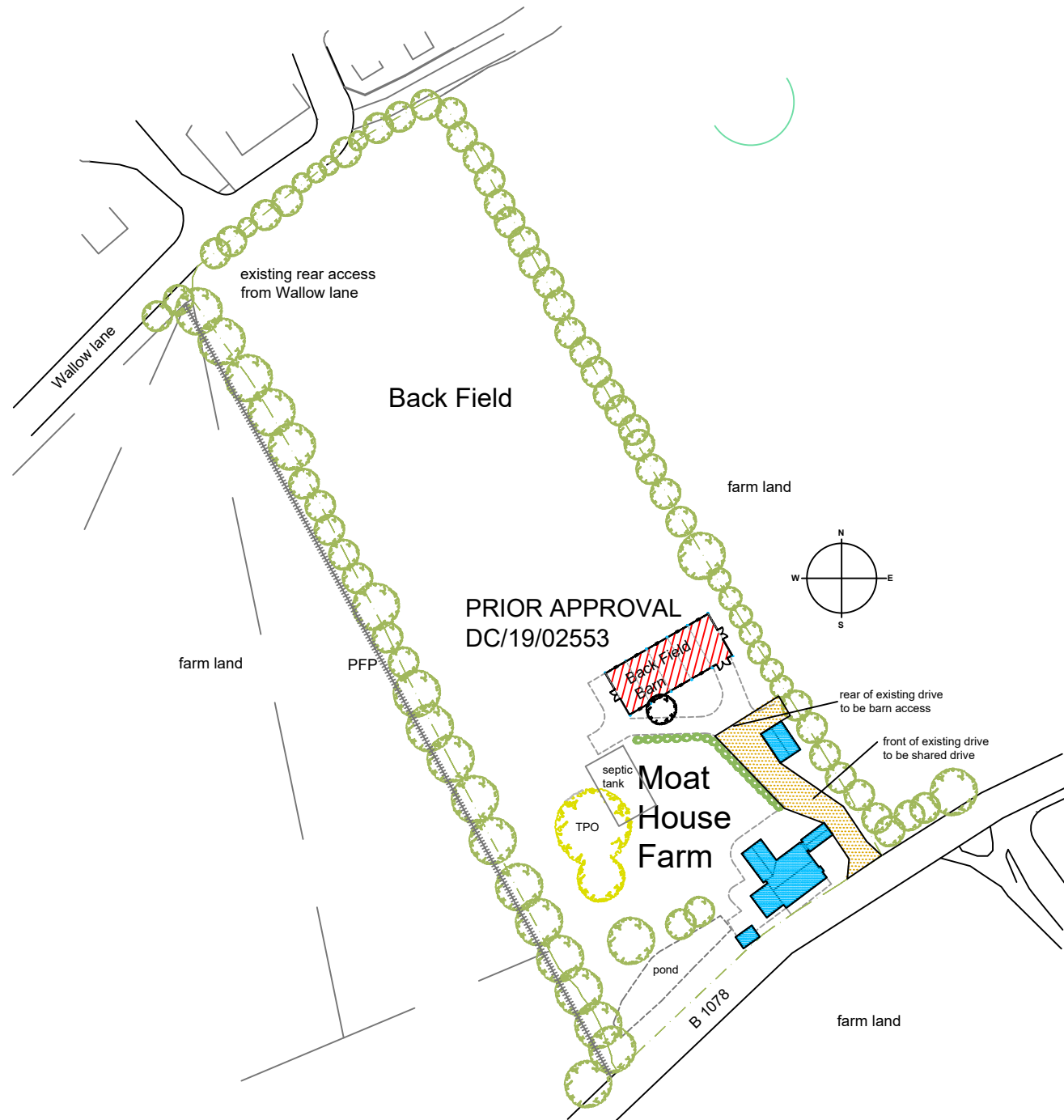
SITE PLAN EXISTING 1:1250 PRIOR APPROVAL SITE PLAN FOR REFERENCE ONLY
