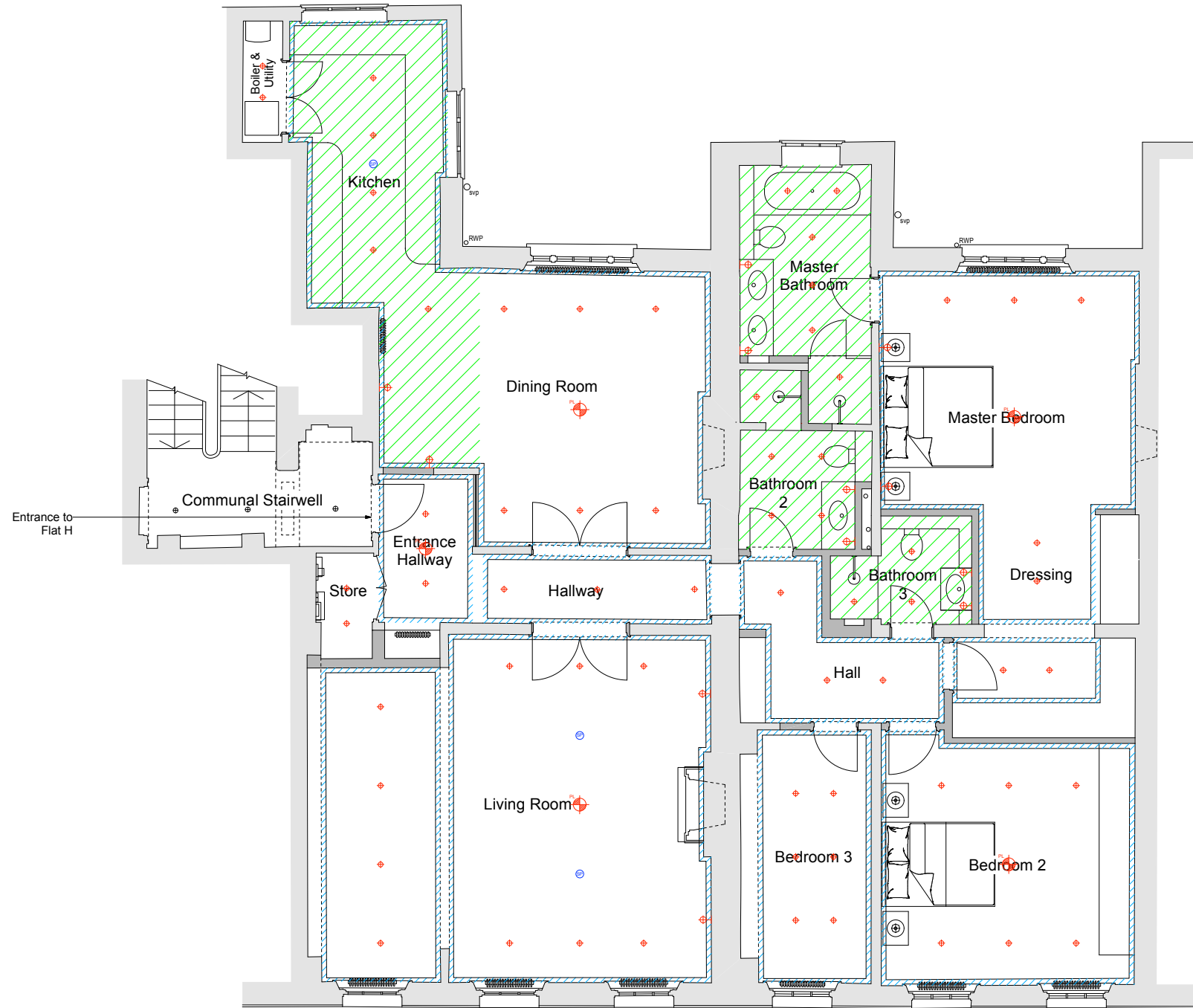
Proposed Third Floor Reflected Ceiling & Lighting Plan
