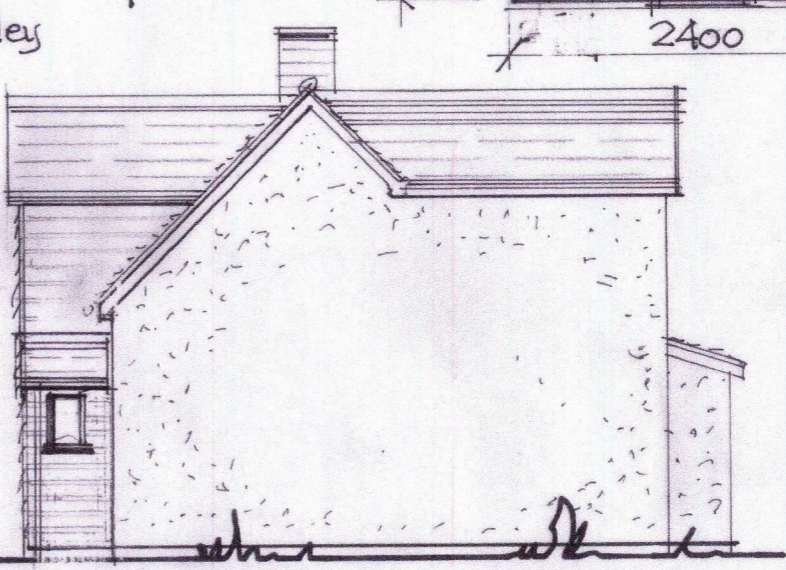
side elevation
