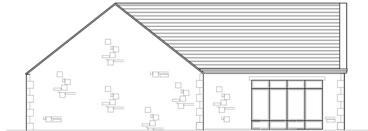
SOUTH ELEVATION AS PROPOSED SCALE: 1/100
