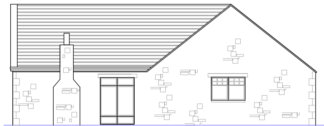
NORTH ELEVATION AS PROPOSED SCALE: 1/100
