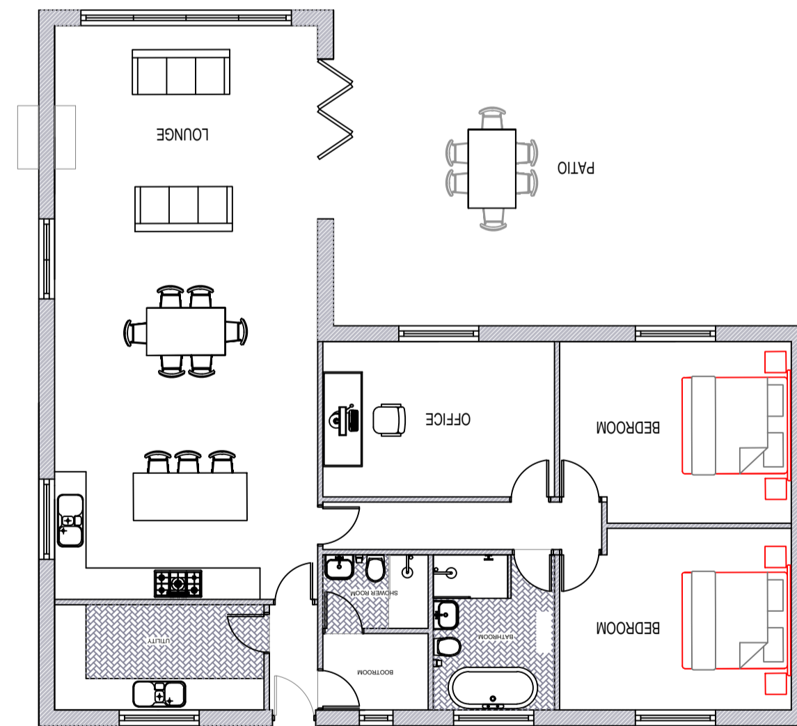
FLOOR PLAN AS PROPOSED SCALE: 1/100
