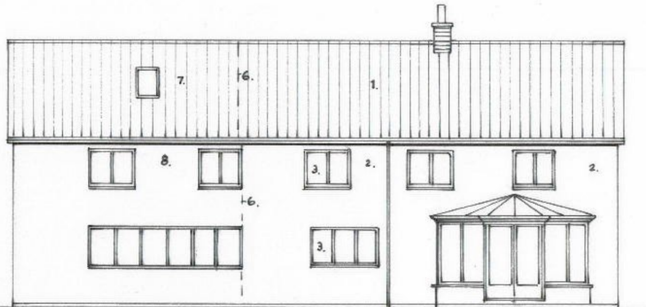
SIDE/SOUTHEAST ELEVATION
