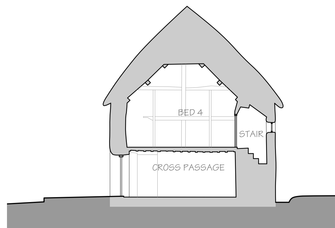
SECTION C-C
