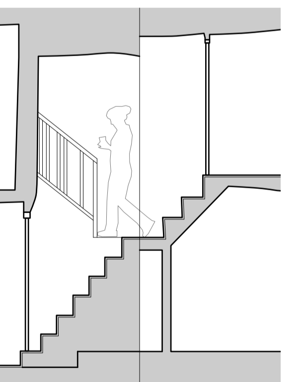
STAIR SECTION
