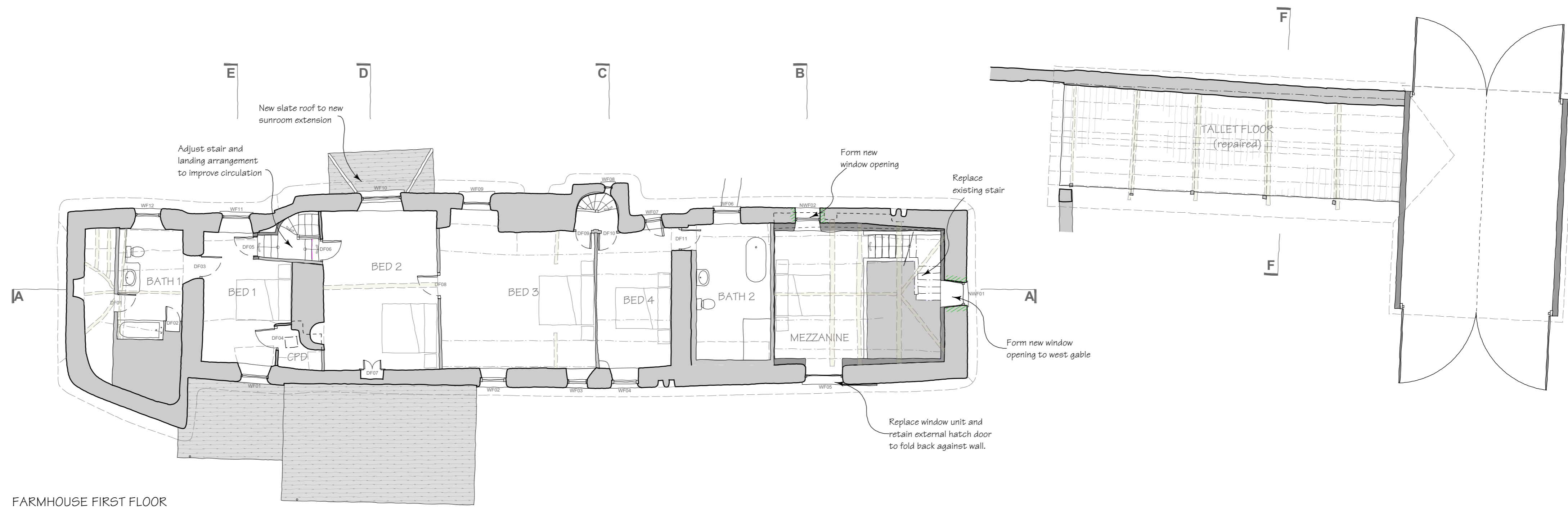
FARMHOUSE FIRST FLOOR
