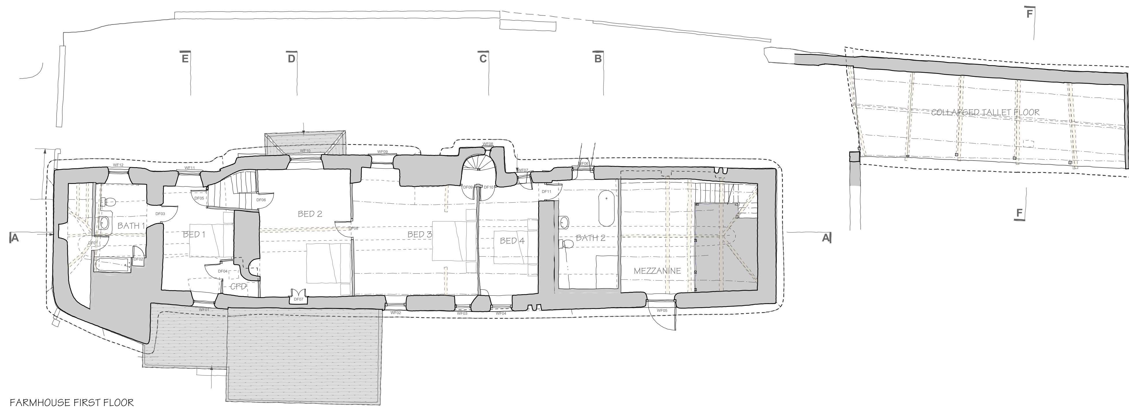
FARMHOUSE FIRST FLOOR
