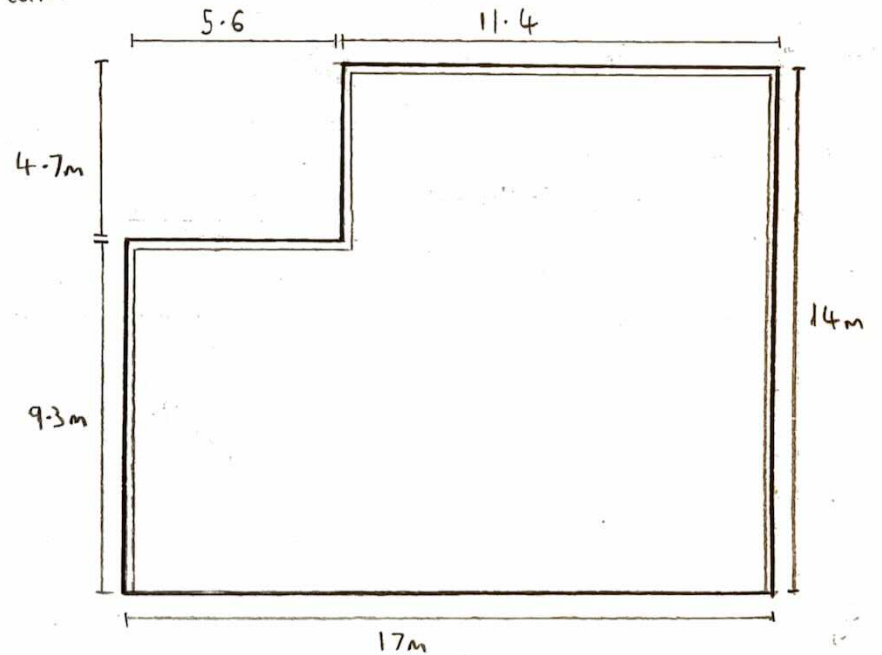
Floor Plan:
