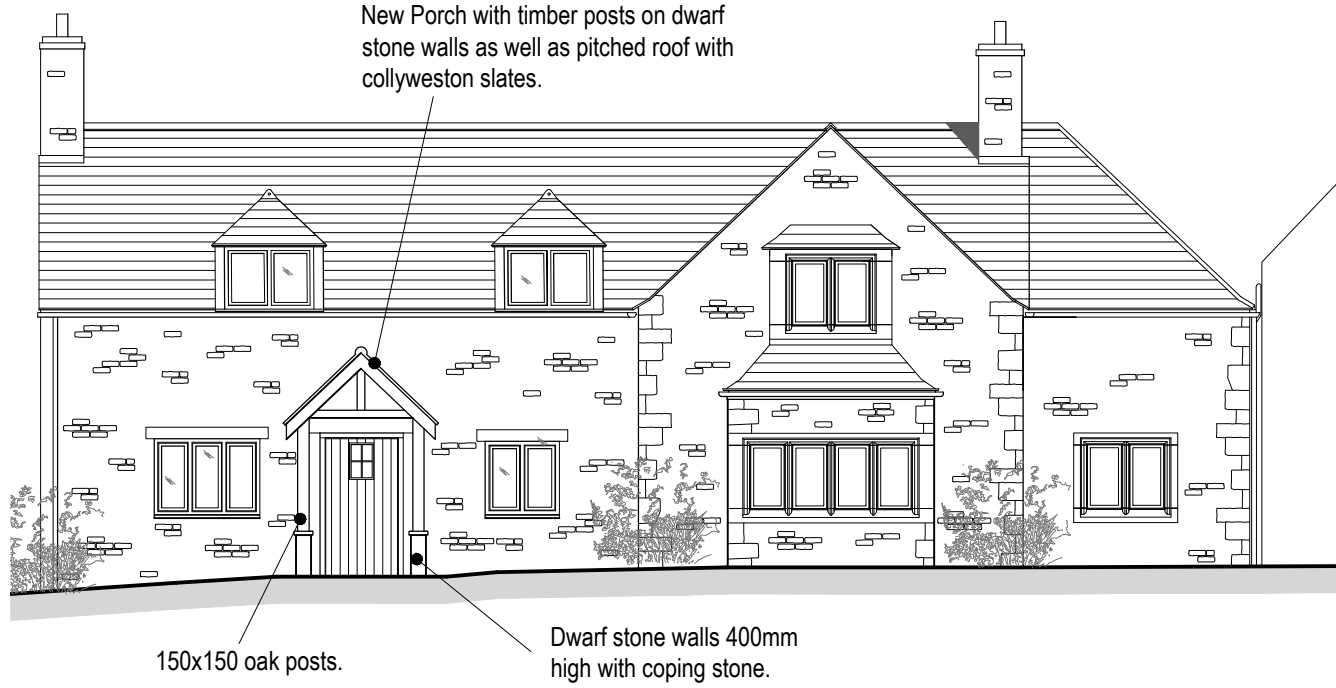
Proposed South (Front) Elevation 1:50 @ A1
