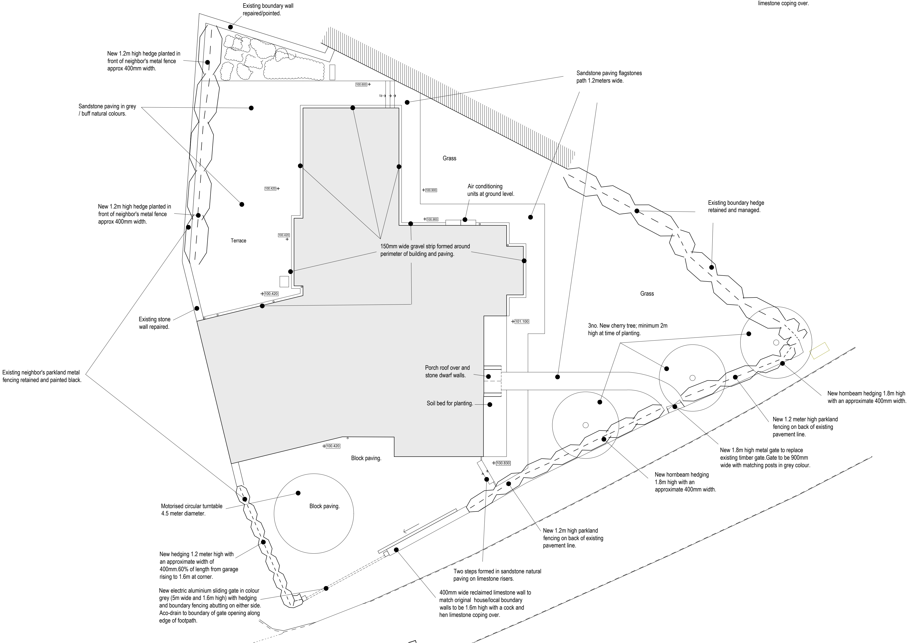
Proposed Landscaping 1:100 @ A1
