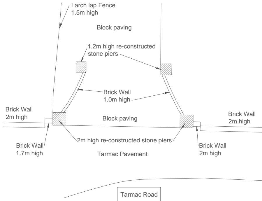
Existing Site Entrance - Plan
