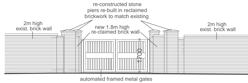
Proposed Site Entrance - Elevation
