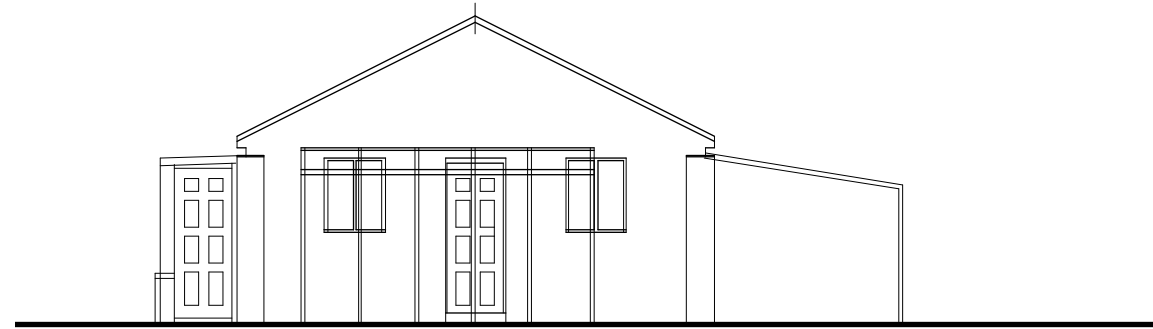
Existing South East Elevation
