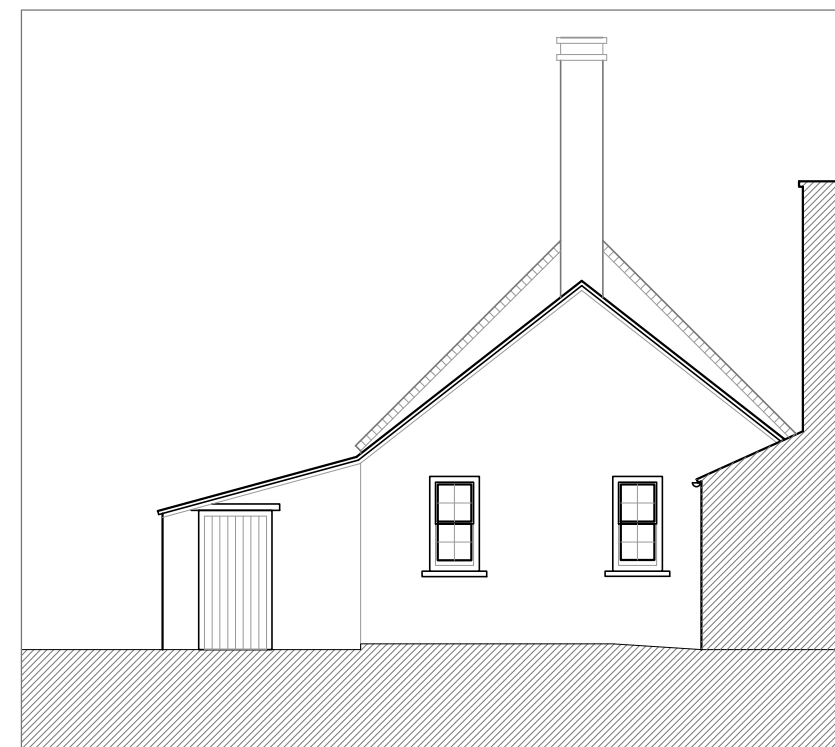
Proposed South Elevation 1:100
