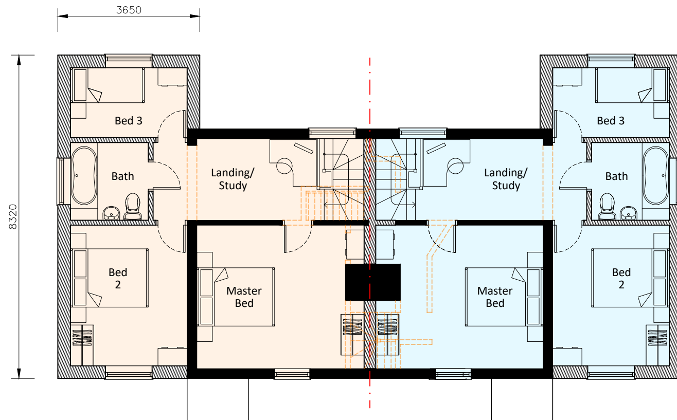
1st Floor Plan as Proposed
