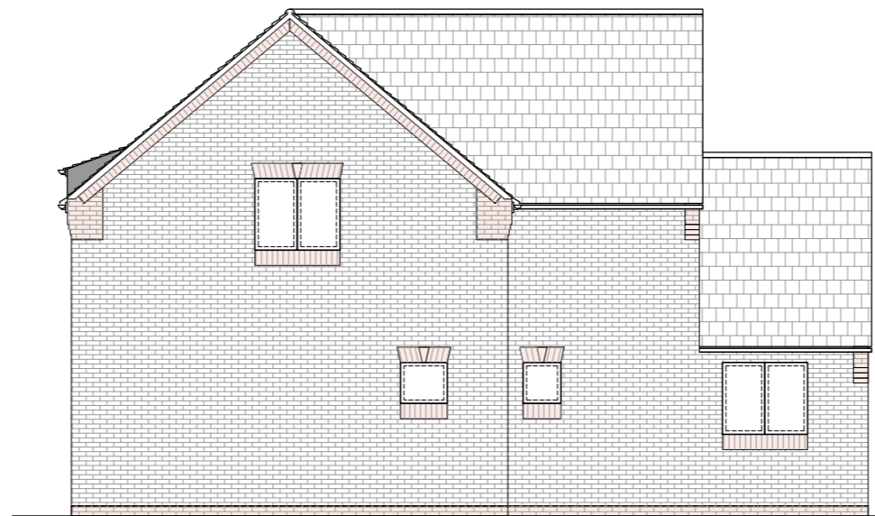
SIDE ELEVATION
