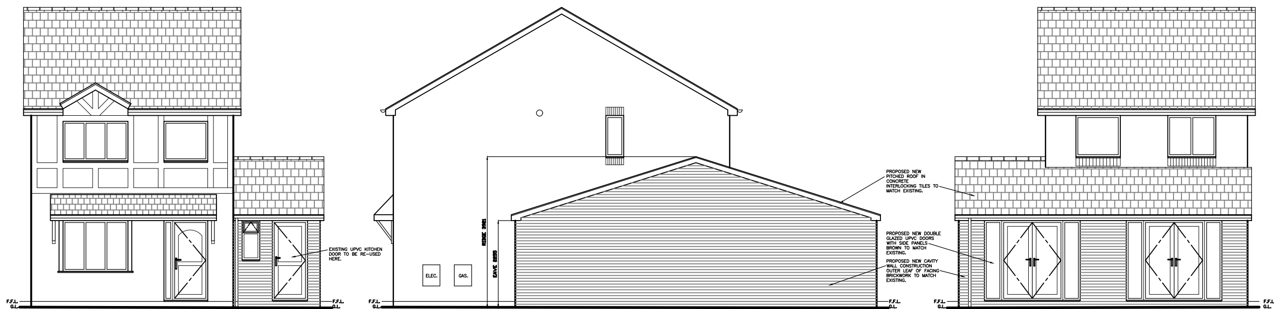
PROPOSED RIGHT SIDE ELEVATION
