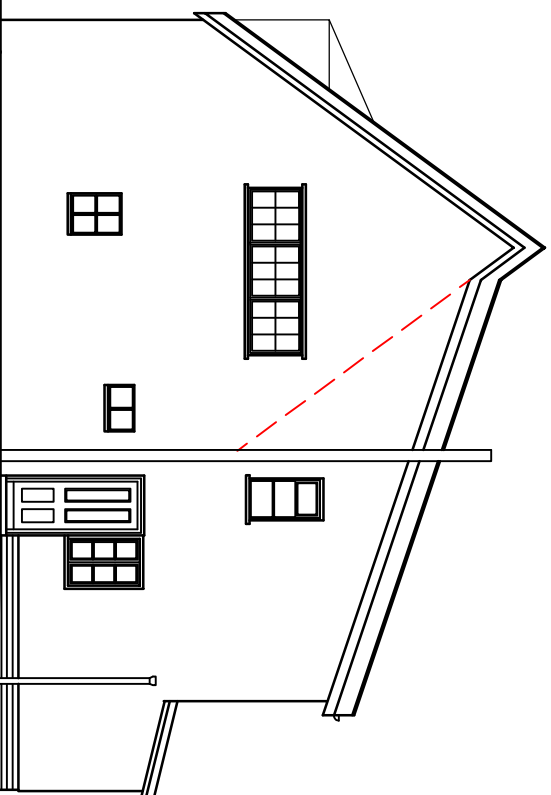
NORTH ELEVATION EXISTING
