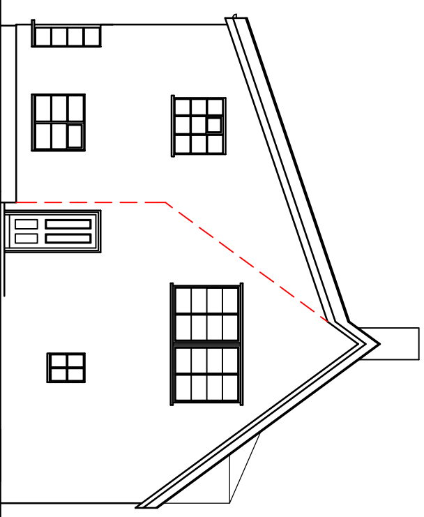
SOUTH ELEVATION EXISTING
