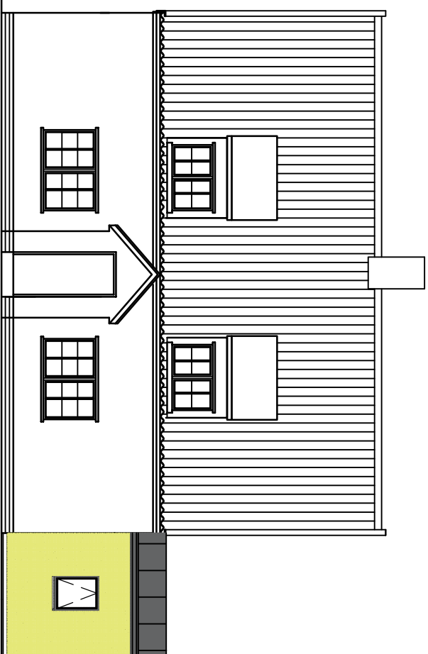
FRONT (EAST) ELEVATION PROPOSED
