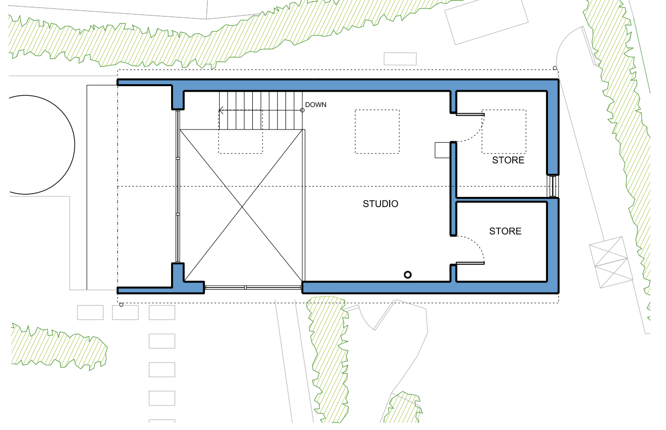
2 1:50 @ A1, 1:100 @ A3 PROPOSED MEZZANINE FLOOR PLAN
