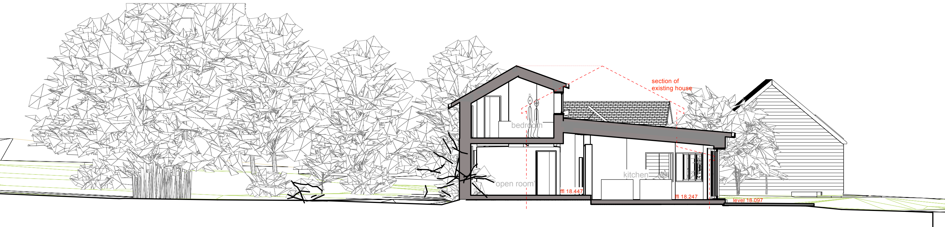
New House Cross Section 1 1:100
