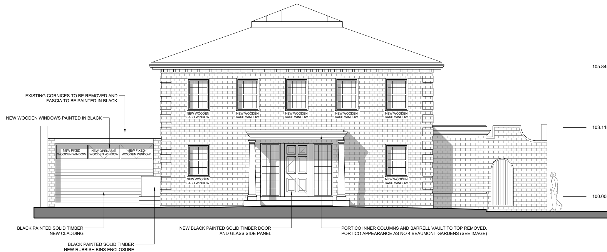
1 NORTH ELEVATION - PROPOSED_ SCALE 1:100 @ A3
