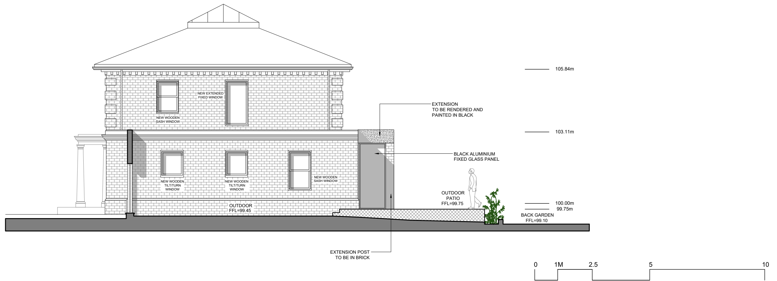
1 WEST ELEVATION - PROPOSED_ SCALE 1:100 @ A3
