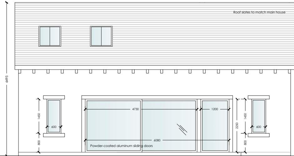
REAR ELEVATION Proposed 1:100@A3
