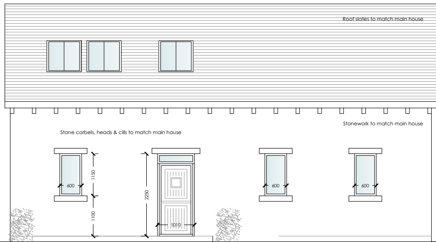
FRONT ELEVATION Proposed 1:100@A3
