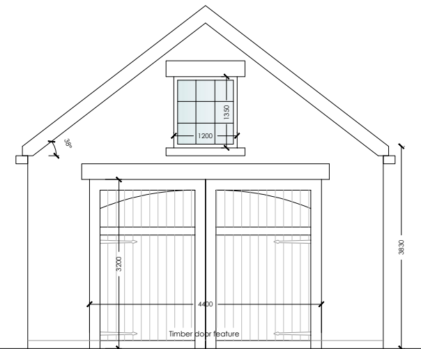
SIDE ELEVATION Proposed 1:100@A3
