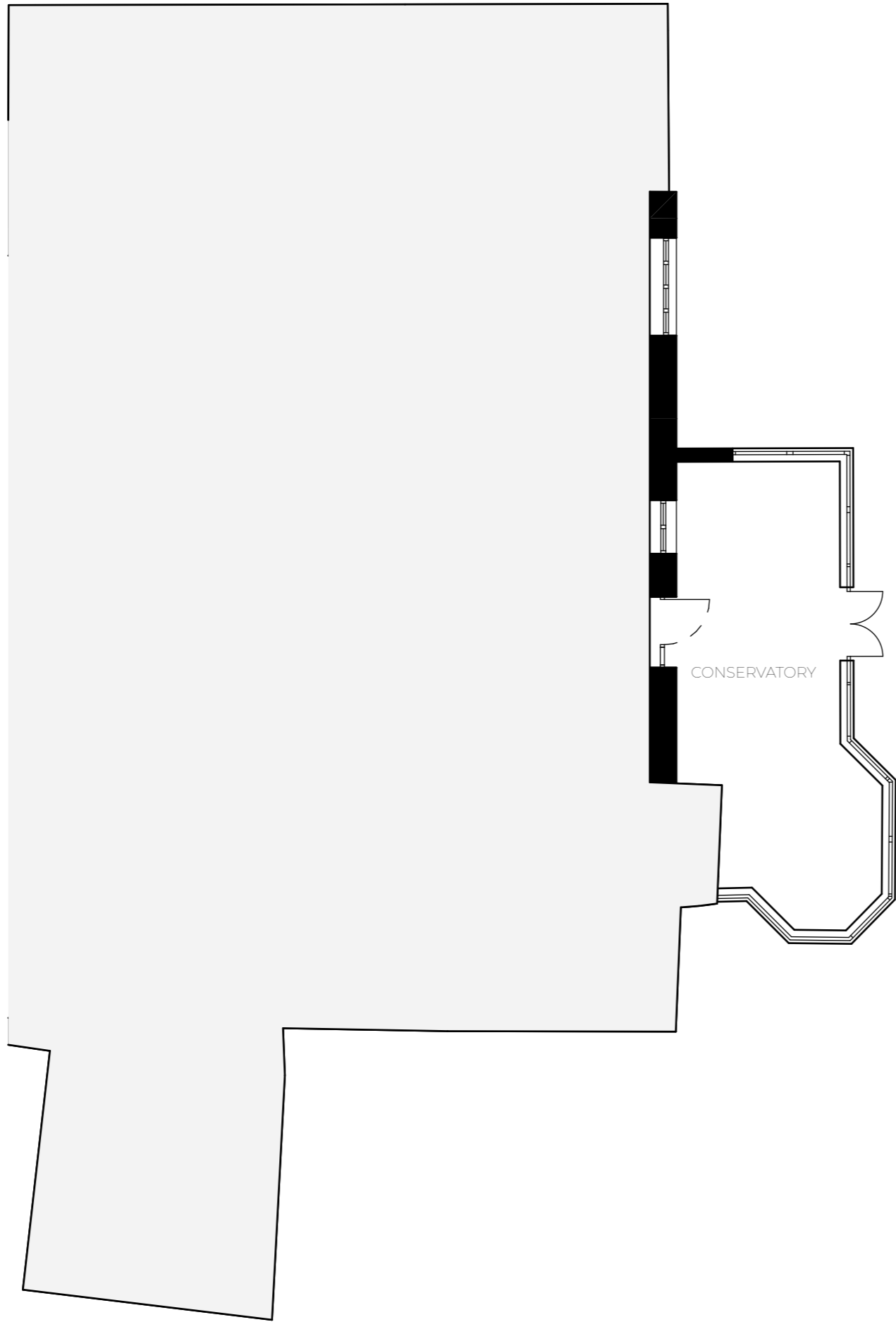
EXISTING GROUND FLOOR 1:100
