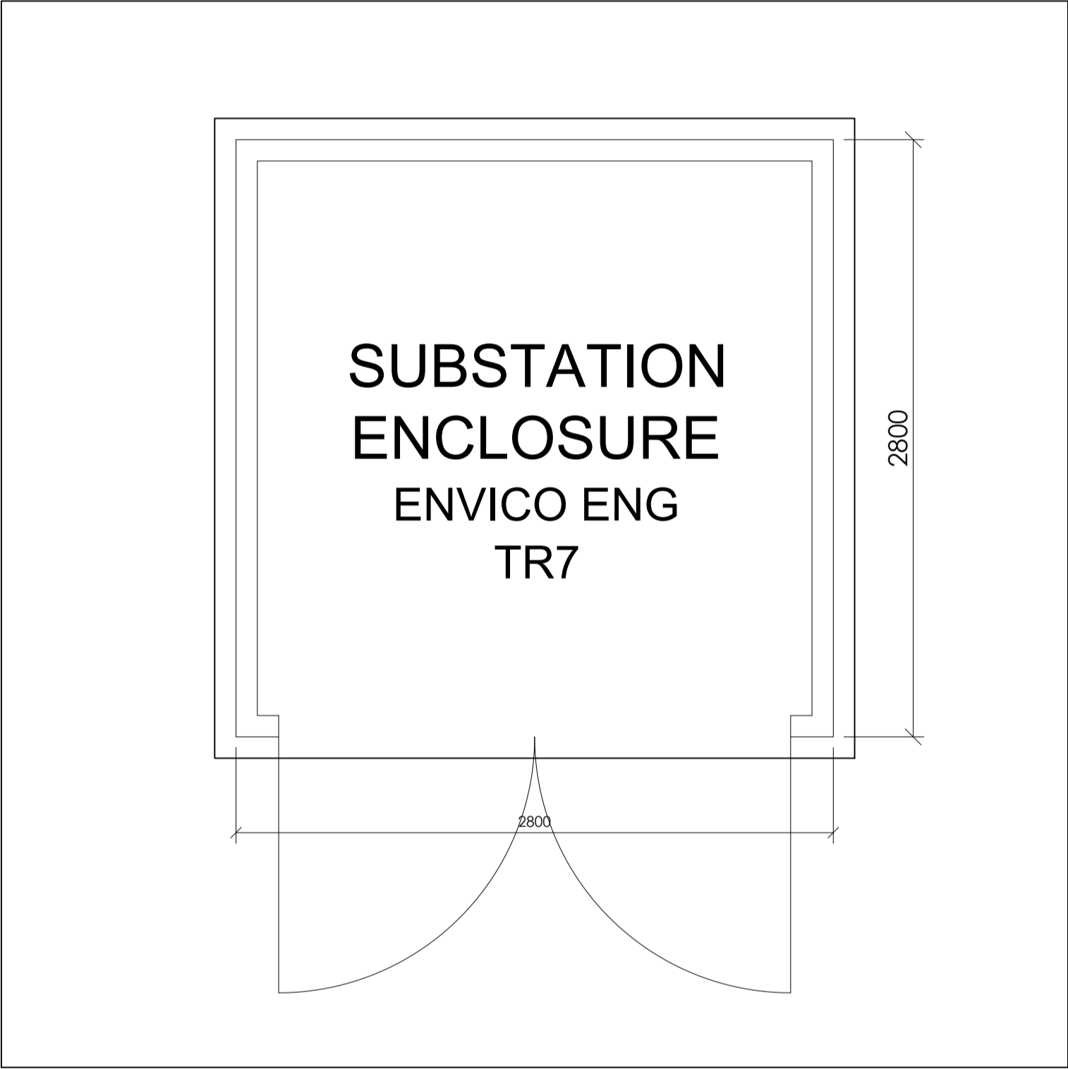
Plan - Substation
