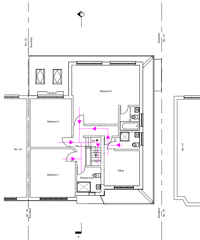
2 Proposed First Floor Fire Safety 1 : 200
