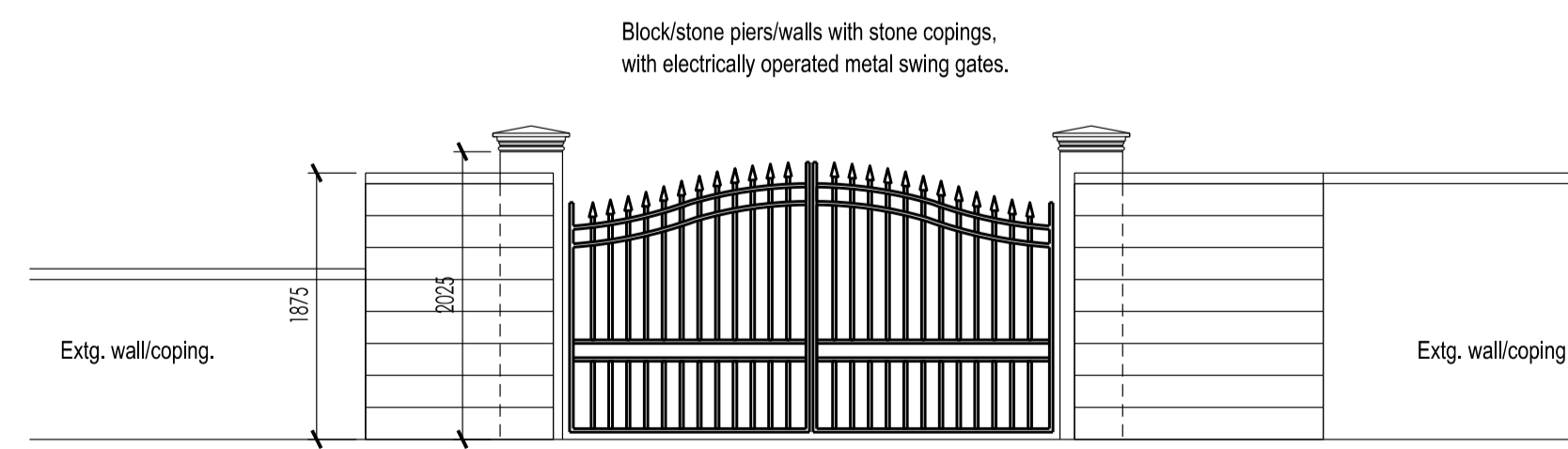
ENTRANCE GATE & WALLS. (1:50)
