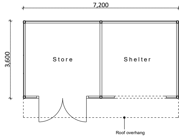
Floor Plan
