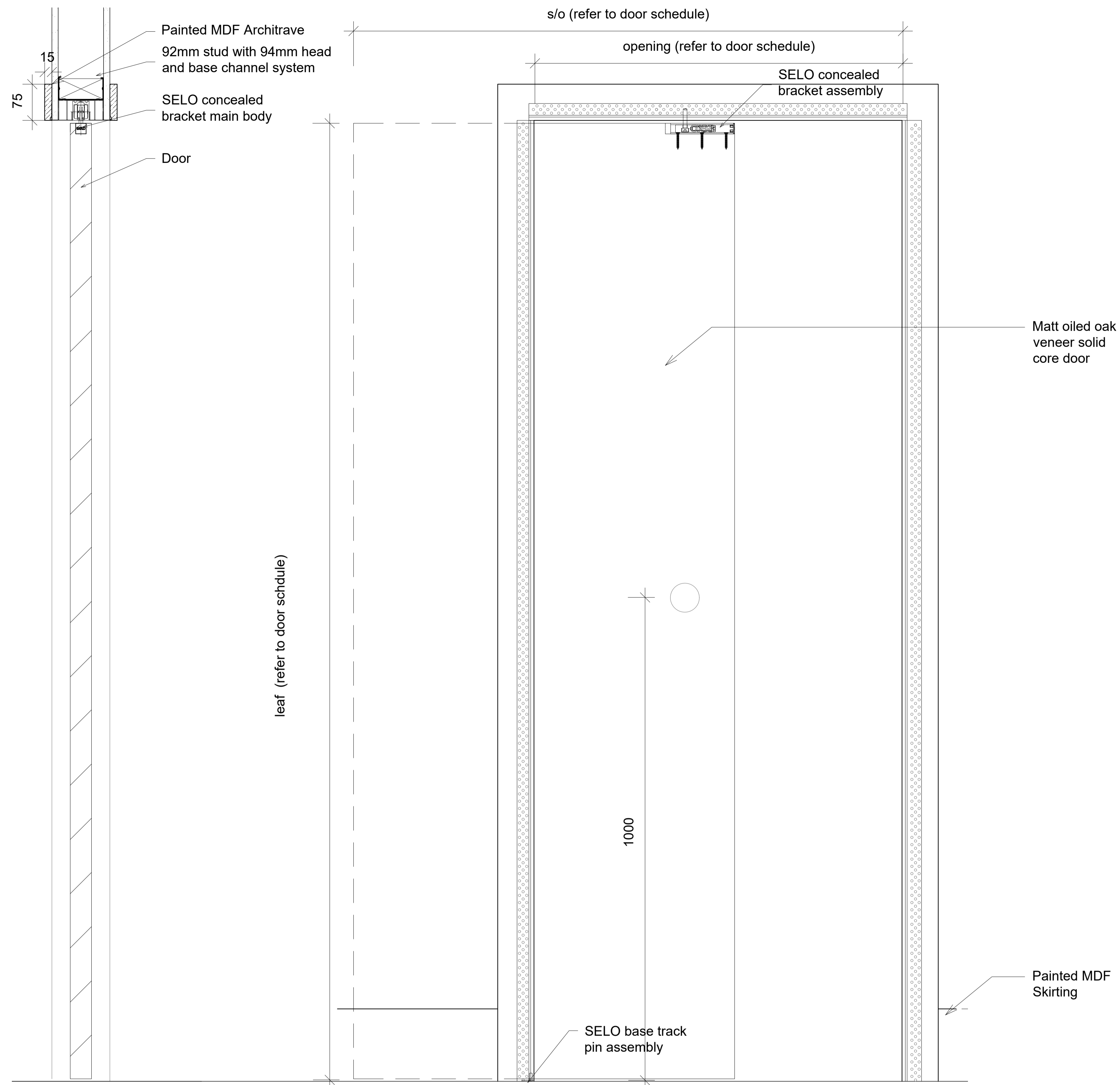
Elev 1 INTERNAL SLIDING POCKET DOOR Scale 1:5@A1
