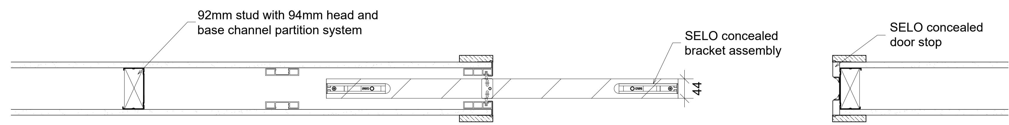
Plan 2 INTERNAL SLIDING POCKET DOOR Scale 1:5@A1
