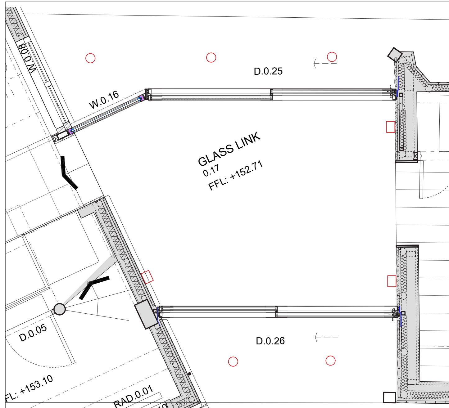
Fig. 6 Positions of lighting to Glazed Link
