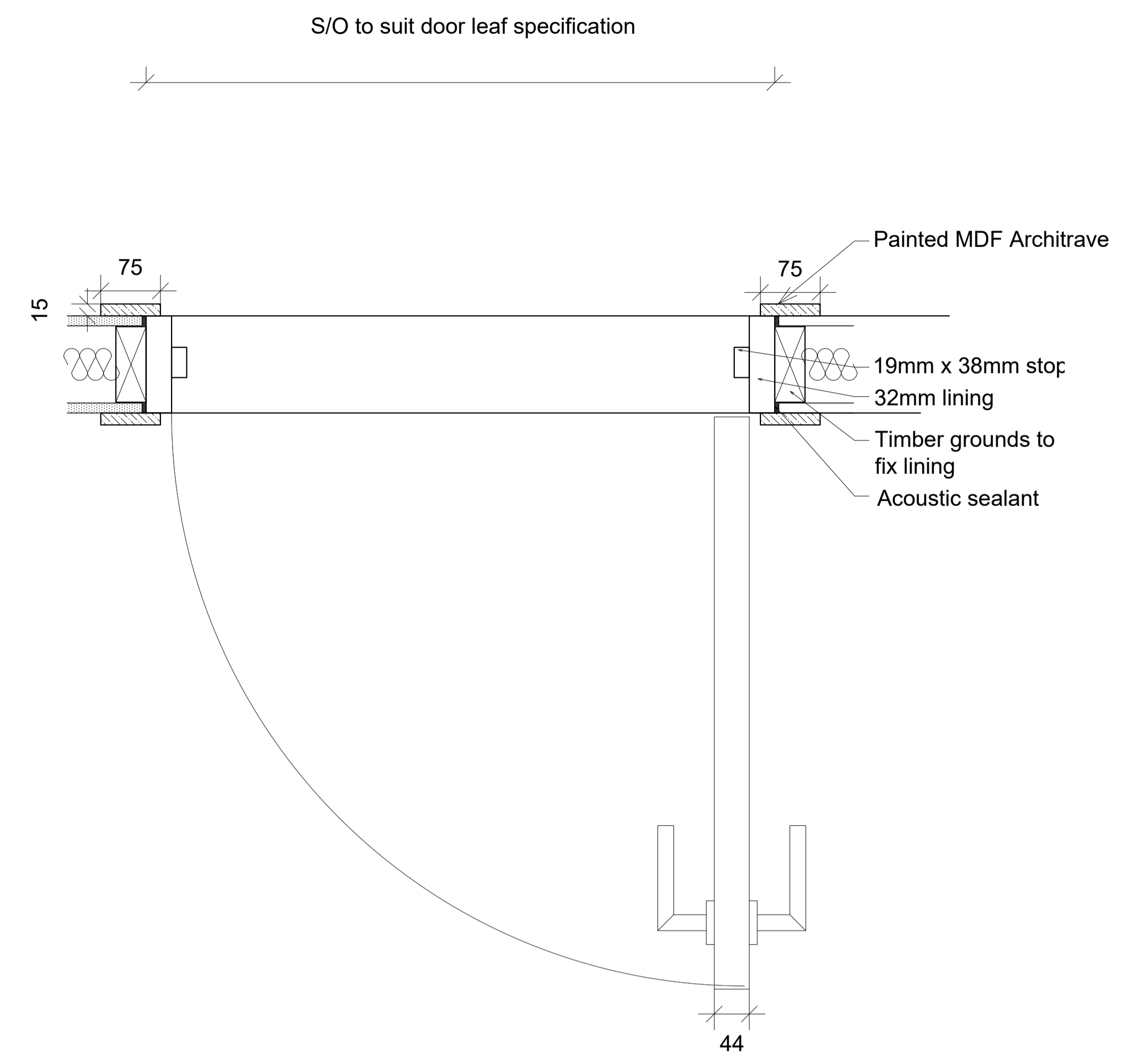
Plan 2 INTERNAL SINGLE DOOR Scale 1:5@A1
