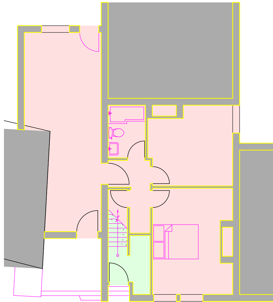
Ground Floor Proposed
