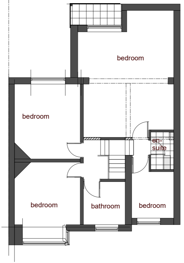
first floor layouts
