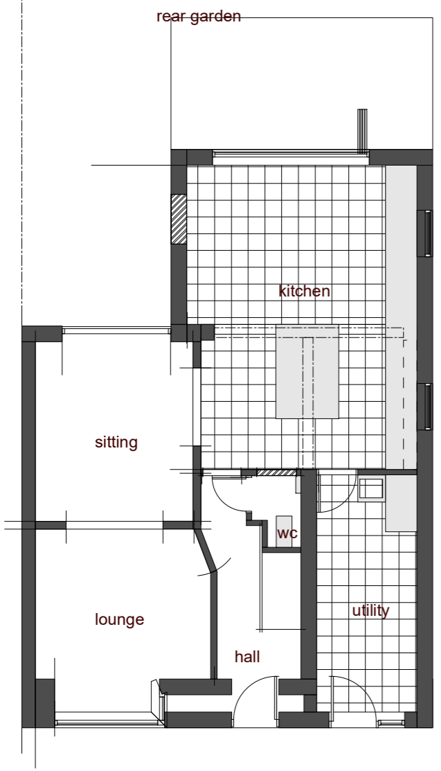
ground floor layouts
