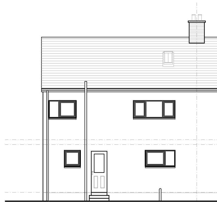
ex. Rear Elevation
