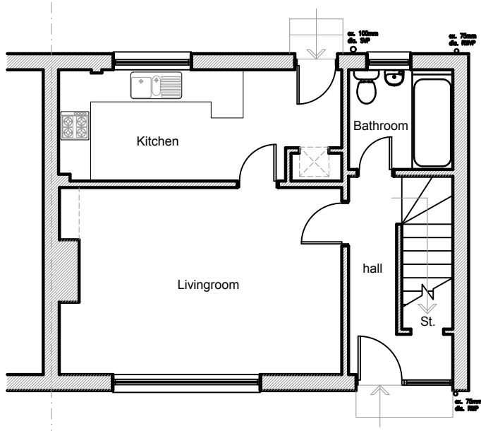
ex. Ground Floor Plan
