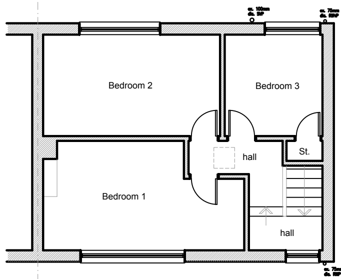
ex. First Floor Plan
