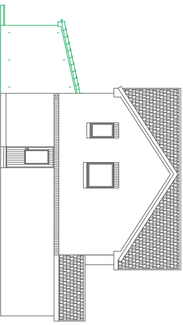
Proposed North Elevation Scale:- 1:100
