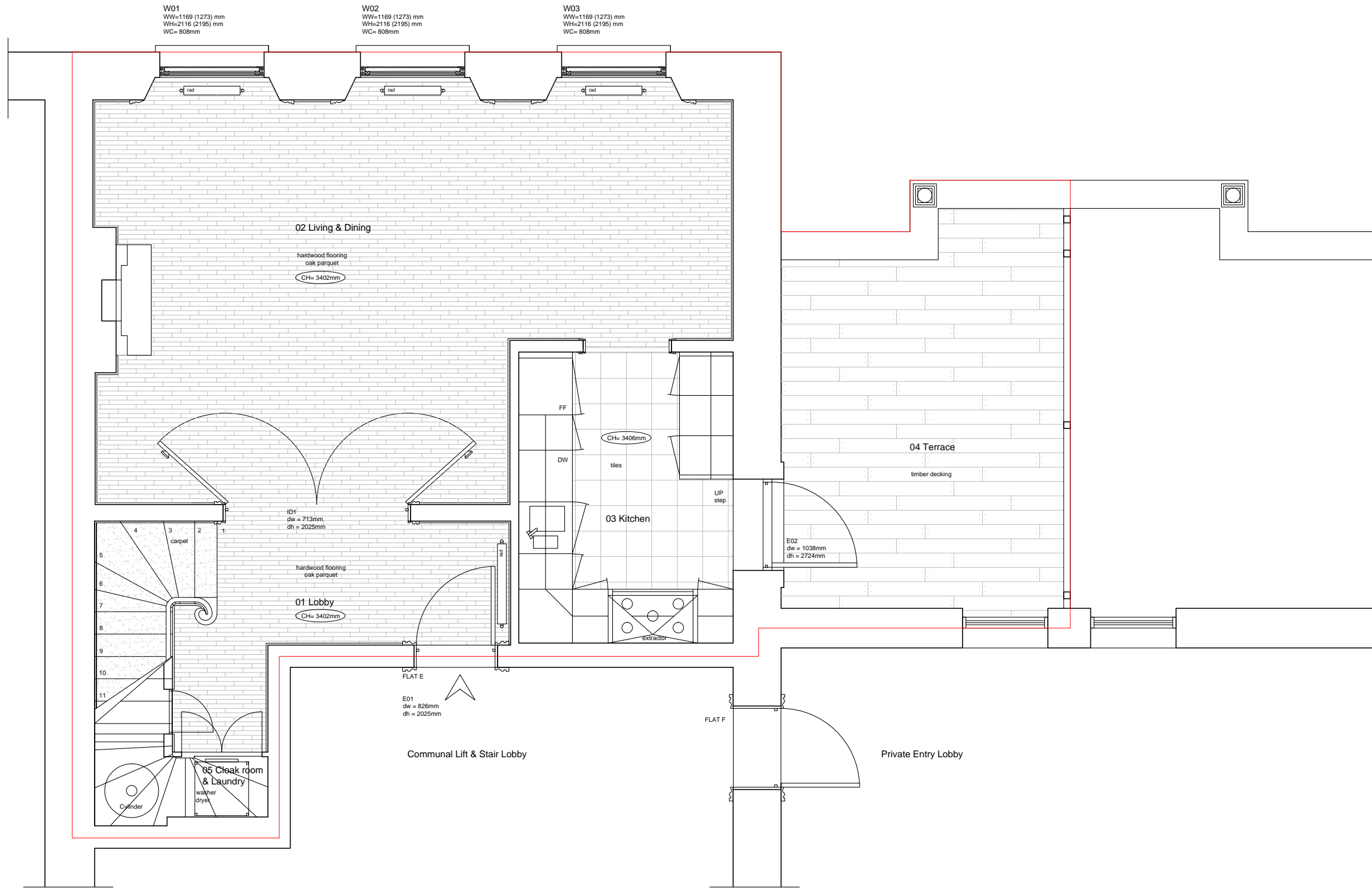
1 Existing Second Floor SCALE 1:50
